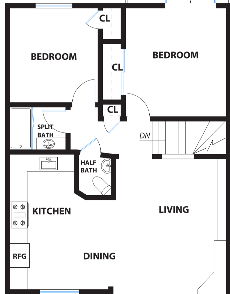
MAIN FLOOR
